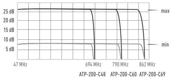
Graphs of gain control
